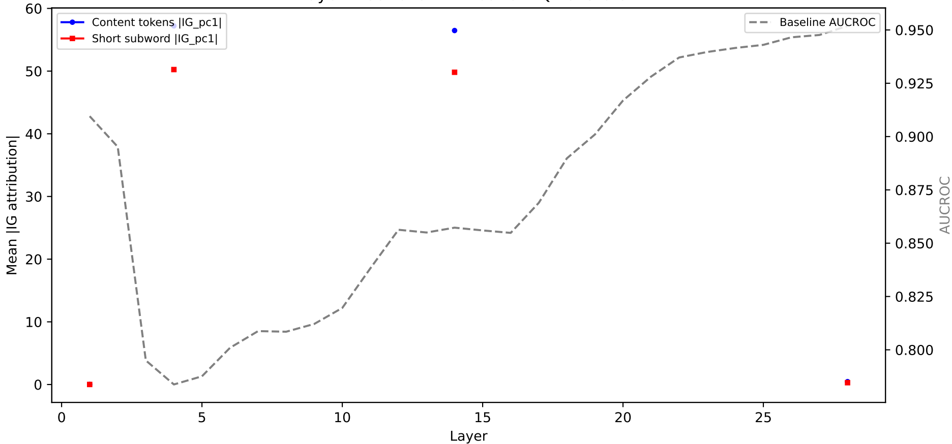
Layer-wise Token Attribution: Qwen3-0.6B
