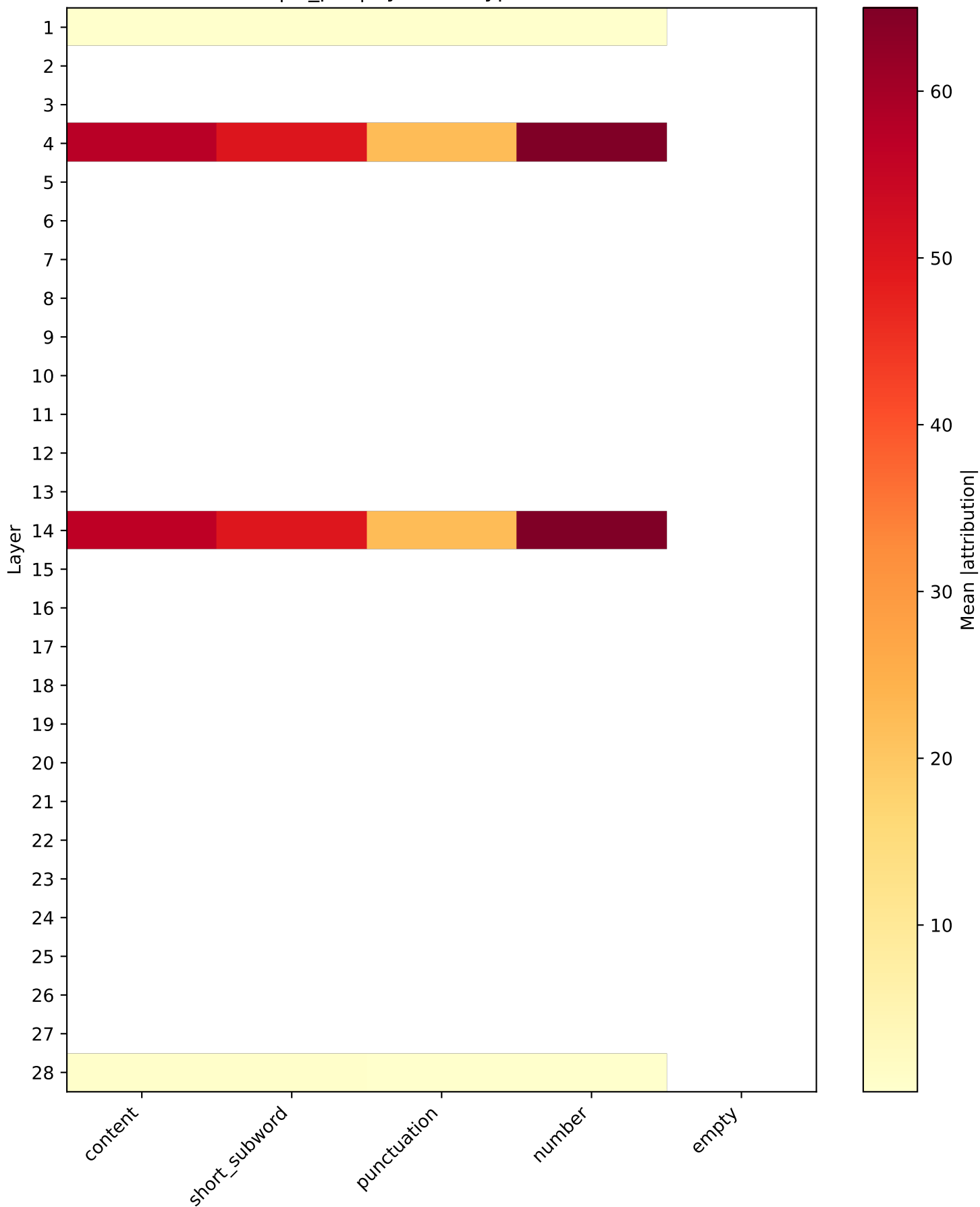
Mean |IG\_pc1| by Token Type: Qwen3-0.6B
