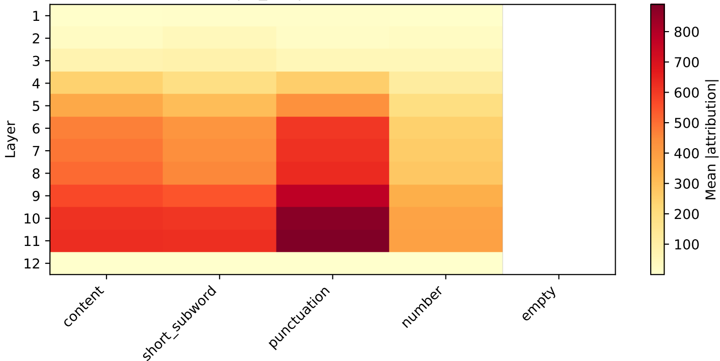
Mean |IG_pc1| by Token Type: PhilTa
