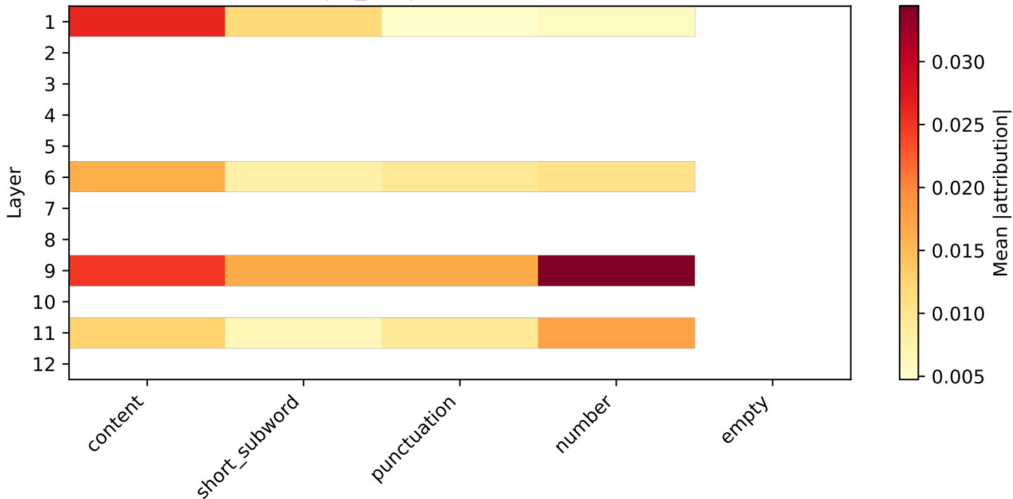
Mean |IG\_pc1| by Token Type: LaBSE
