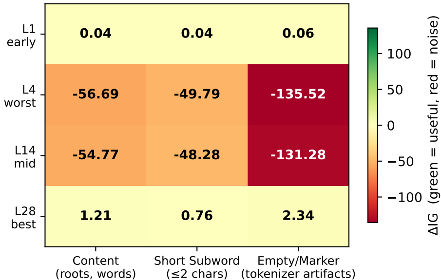
\Delta IG Heatmap — Qwen3-0.6B
