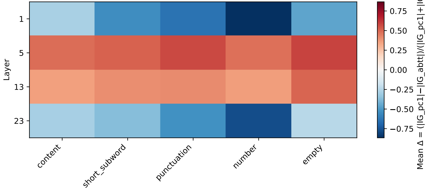
Attribution Delta by Token Type: KaLM-mini (+) = more PC1 noise, (-) = more ABTT signal
