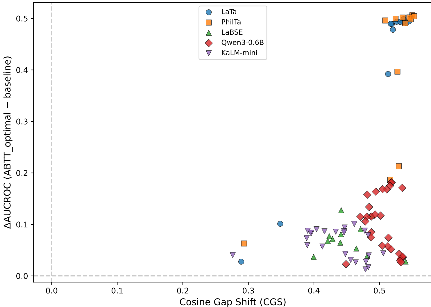
CGS vs \Delta AUCROC (Spearman \rho = +0.478 , p = 2.5e-06 )
