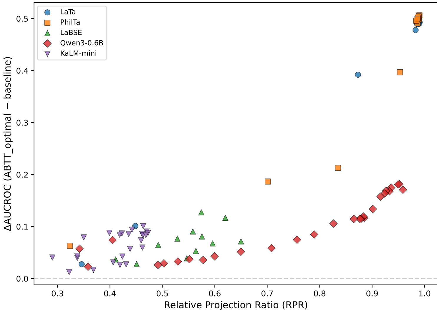
RPR vs \Delta AUCROC (Spearman \rho = +0.834 , p = 6.1e-24 )
