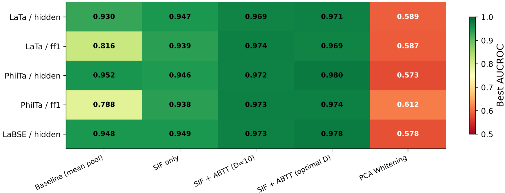
Best AUCROC by Model/Representation and Method
