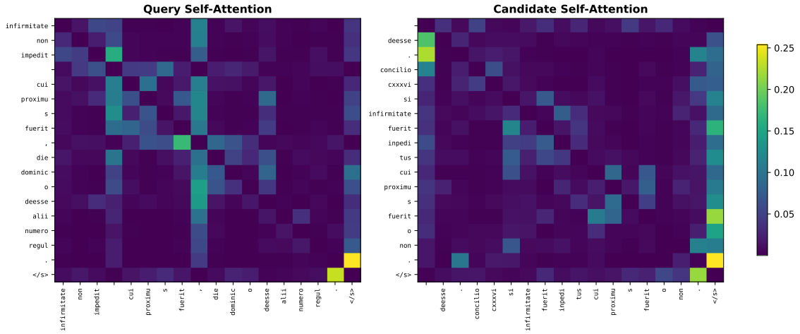
Figure 7: Companion self-attention maps for the same PhilTa example. ABTT is applied after encoding, so attention is included only as supporting context.
