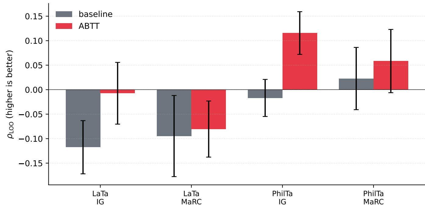
\rho_{\text{LOO}} improves under ABTT (T5 models; main-text scope)
