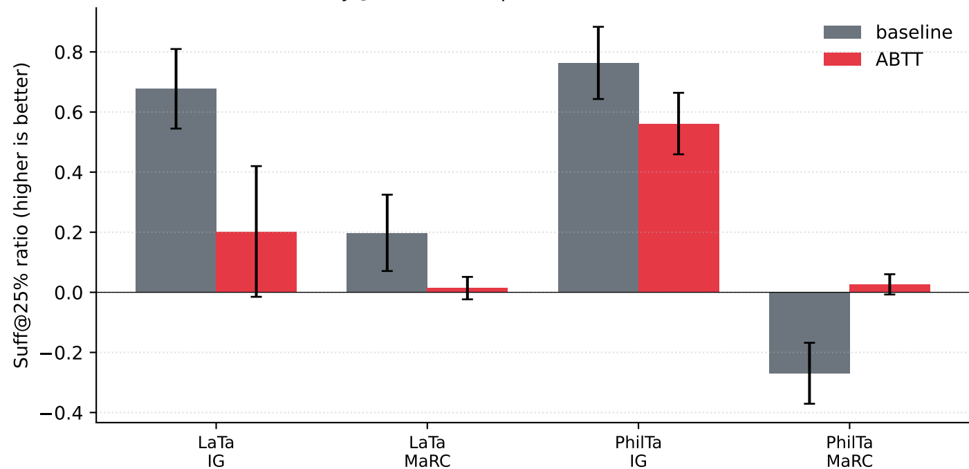
Sufficiency@25%: mixed picture under ABTT (T5 models)
