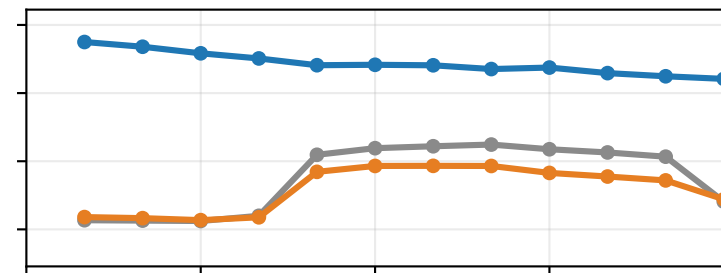
mT5-base
