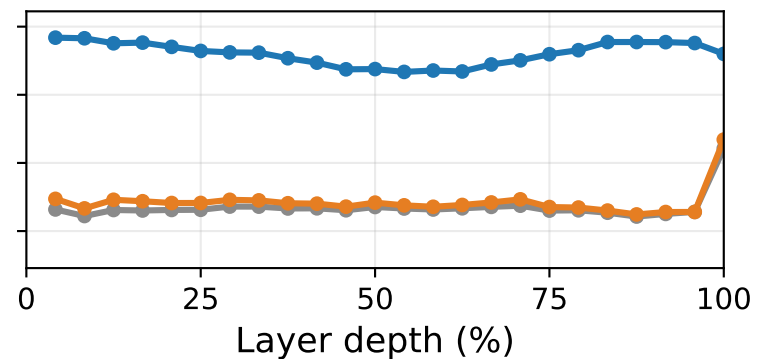
KaLM-mini
