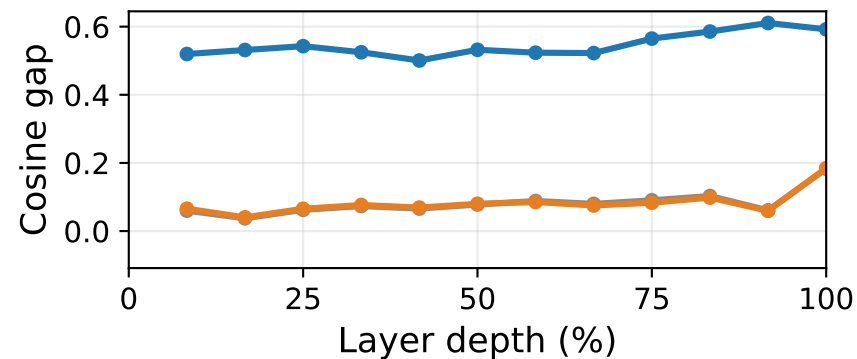
LaBSE
