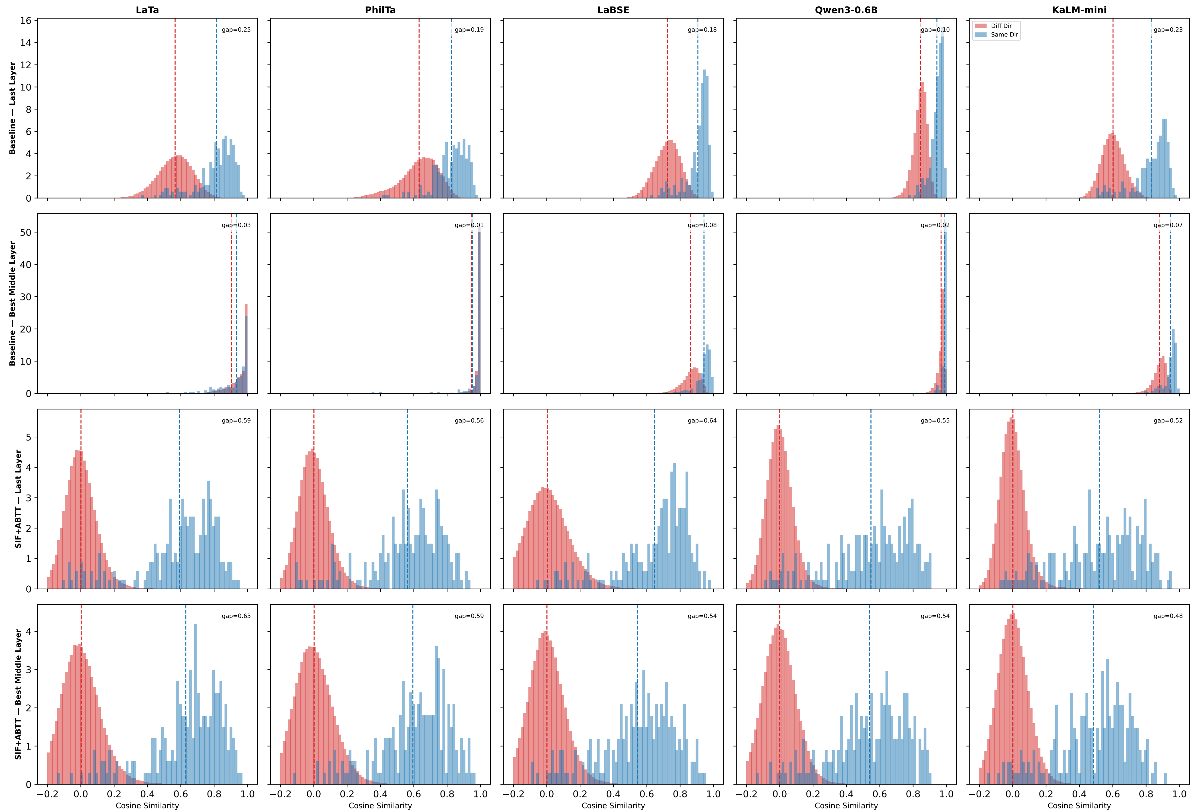
Fig 5: Cosine Similarity Distributions — 4 Conditions Compared
