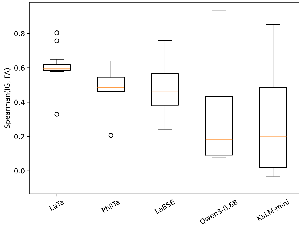
IG-FA Agreement: pc1_dot
