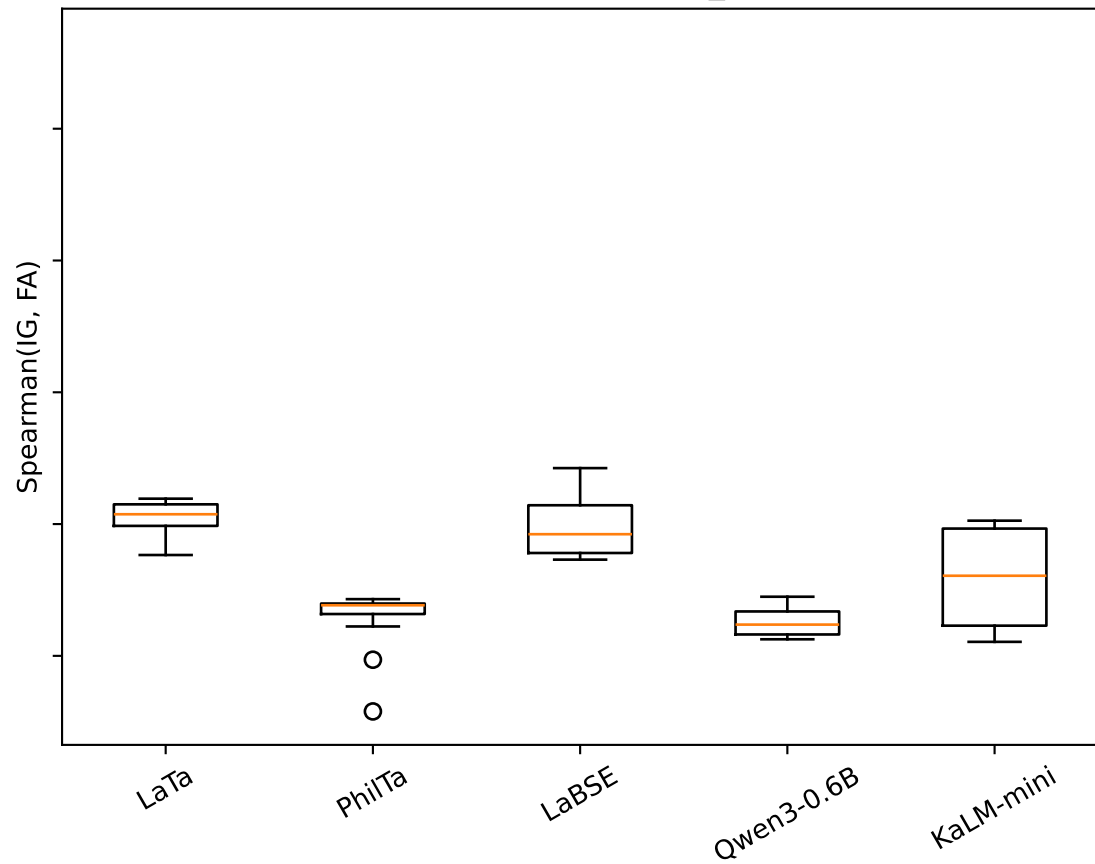
IG-FA Agreement: abtt_norm
