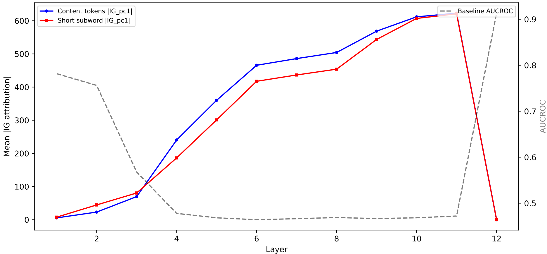
Layer-wise Token Attribution: PhilTa
