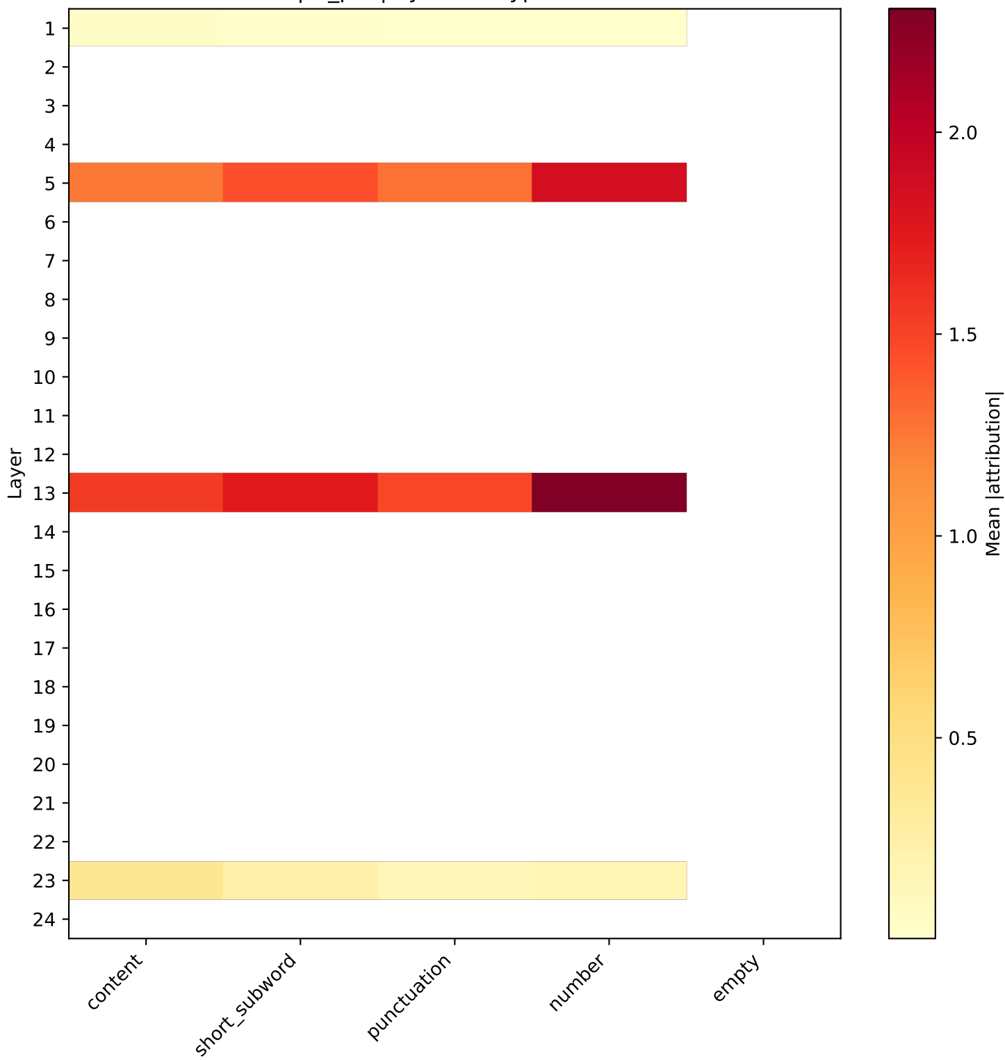
Mean |IG\_pc1| by Token Type: KaLM-mini
