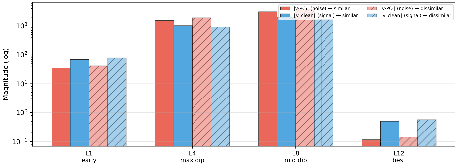
PhilTa — PC 1 Noise vs Clean Signal
