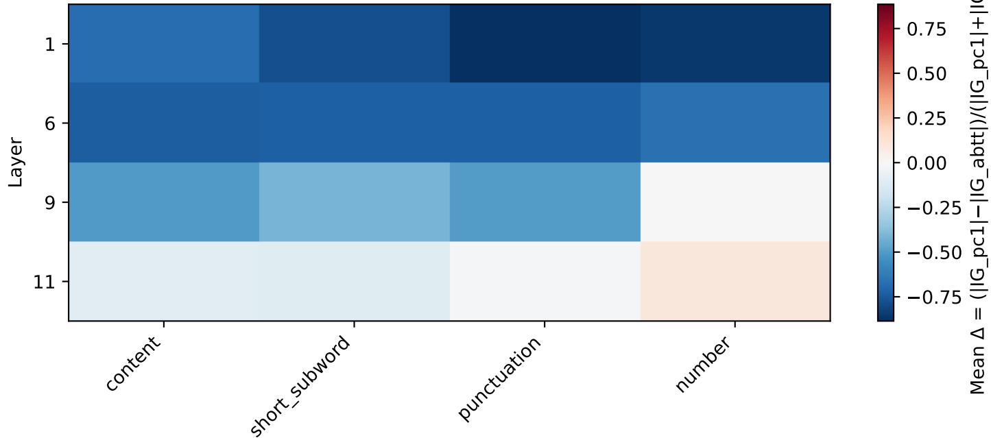
Attribution Delta by Token Type: LaBSE (+) = more PC1 noise, (−) = more ABTT signal
