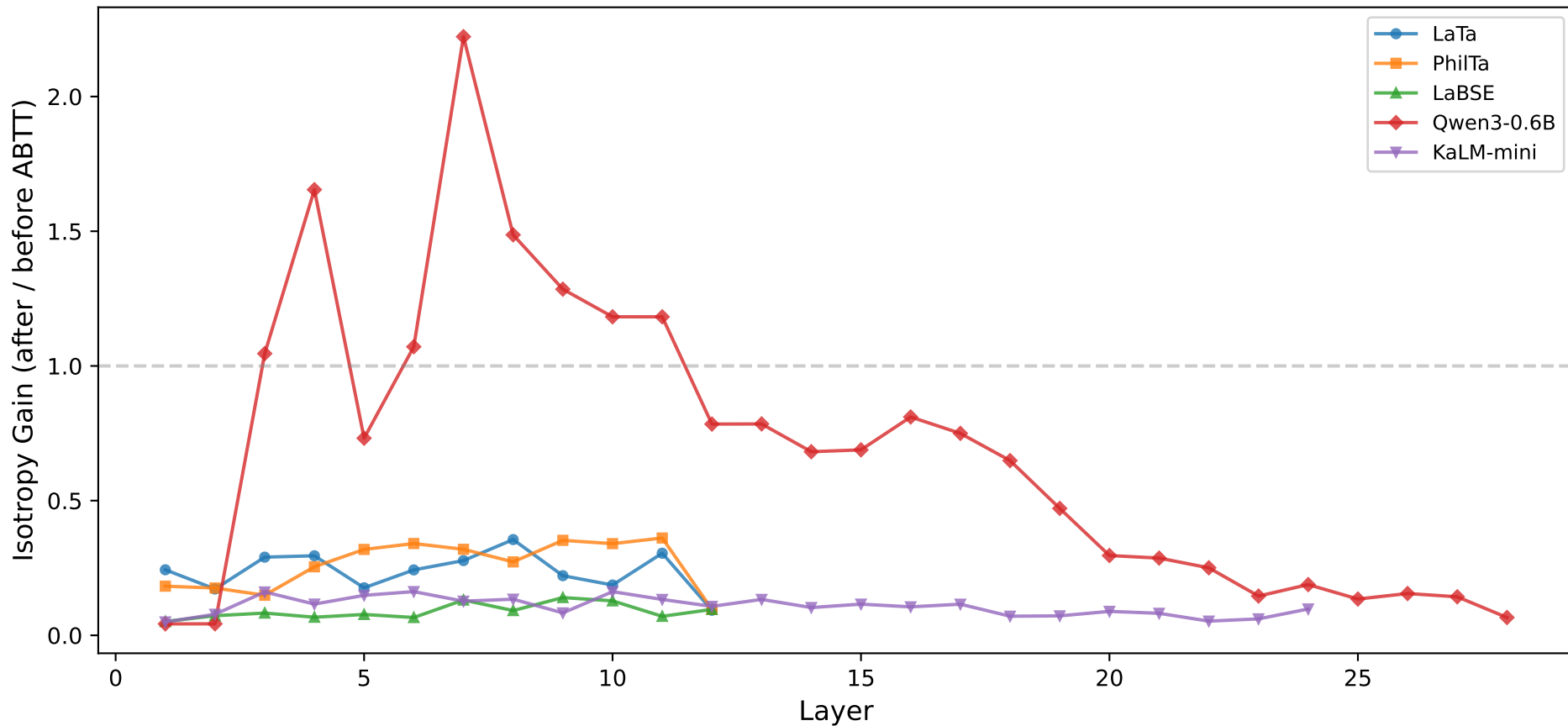
Isotropy Gain by Layer
