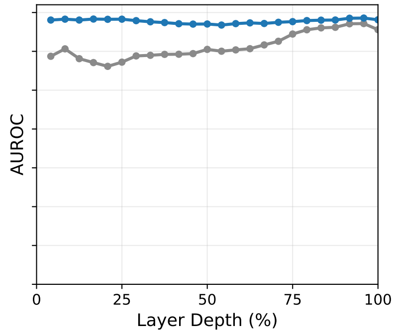
KaLM-mini
