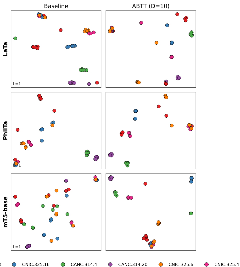
Figure 8: t-SNE projections of the 1,705 labelled fragments at each model's selected layer for LaTa, PhilTa, and mT5-base. Columns compare baseline mean pooling with pure ABTT using D = 10 . Colors mark the six most-populated directories.
