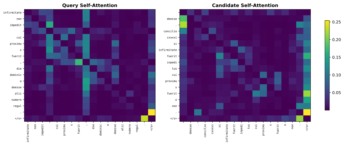
Figure 6: Companion self-attention maps for the same PhilTa example as Figure 5. ABTT is applied after encoding, so attention is included only as supporting context.
