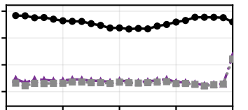
KaLM-mini
