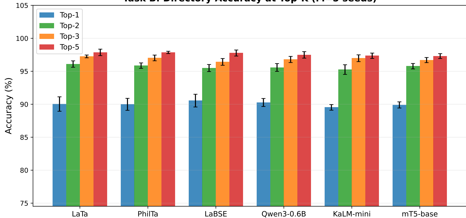
Task B: Directory Accuracy at Top-K (M=5 seeds)
