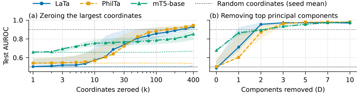
Figure 3: Test ranking AUROC at the 26 collapsed layers of LaTa (10 layers), PhilTa (9) and mT5-base (7); lines: median over a model’s collapsed layers; bands: their range. (a) Zeroing the k coordinates of largest mean absolute value; dotted: k random coordinates (mean of five draws), within 0.001 of the baseline up to k = 10 and within 0.03 at 400. Up to k = 10 (vertical line) the best layer reaches 0.794. (b) Removing the top D principal components ( D = 0 : centering only). Dashed line: AUROC 0.90. All fits use training embeddings.
