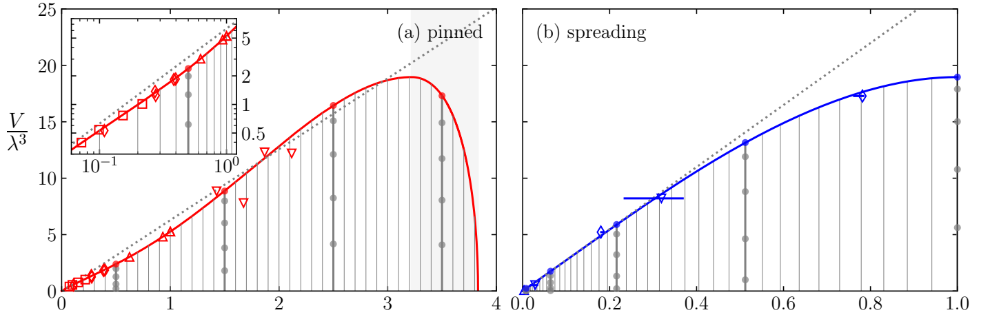
Figure 3 (a) Volume V of pinned bubbles. The solid red line shows the detachment volume as a function of contact radius r_0 , while the dotted grey line, V = 2\pi\lambda^2 r_0 , shows the Tate prediction 10 . Empty symbols denote experimental data: squares 13 , diamonds 14 , down-triangles 15 , and up-triangles 16 . Inset: same data on a logarithmic scale, showing the small-radius range in greater detail. (b) Volume V of spreading bubbles. The solid blue line shows the detachment volume as a function of contact angle \phi_0 , which is cubed to allow comparison with the Fritz 19 prediction V = 0.887\lambda^3 \phi_0^3 (dotted grey line). Symbols denote experimental data: up-triangles 23 , down-triangles 22 , and diamonds 25 ; error bars indicate advancing and receding contact angles. In (a) and (b), vertical grey lines and filled circles show the evolution of bubbles up to detachment.
