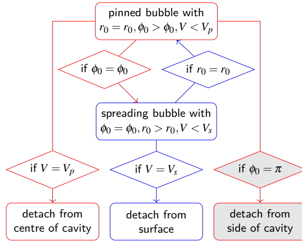
Figure 4 Decision tree for bubble detachment. Red branches correspond to pinned bubbles and blue branches to spreading bubbles. The quantities V_p and V_s denote the corresponding maximum stable bubble volumes, while \phi_0 is the contact angle on the surrounding substrate.
