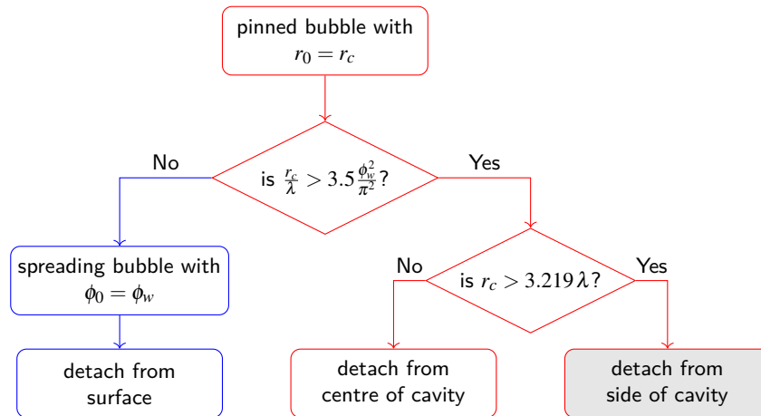
Figure 6 Decision tree for bubble detachment. Red branches correspond to pinned bubbles and blue branches to spreading bubbles. The cavity radius is r_c , and the wetting angle on the surrounding substrate is \phi_w .
