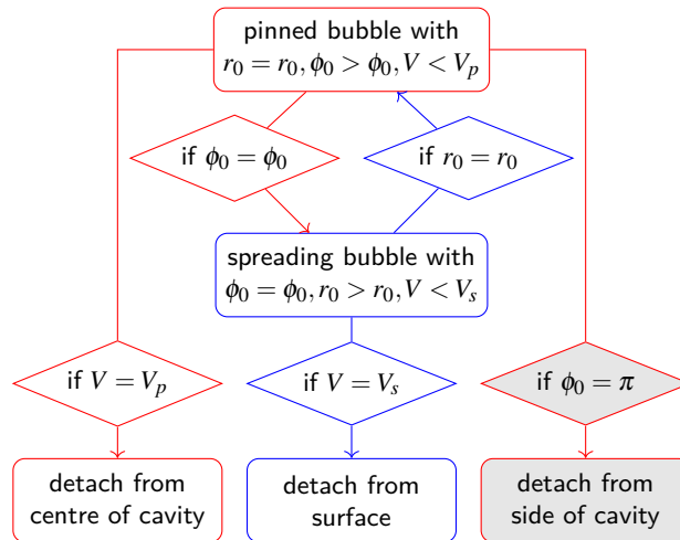
Figure 6 Decision tree for bubble detachment. Red branches correspond to pinned bubbles and blue branches to spreading bubbles. The quantities V_p and V_s denote the corresponding maximum stable bubble volumes, while \phi_0 is the contact angle on the surrounding substrate.
