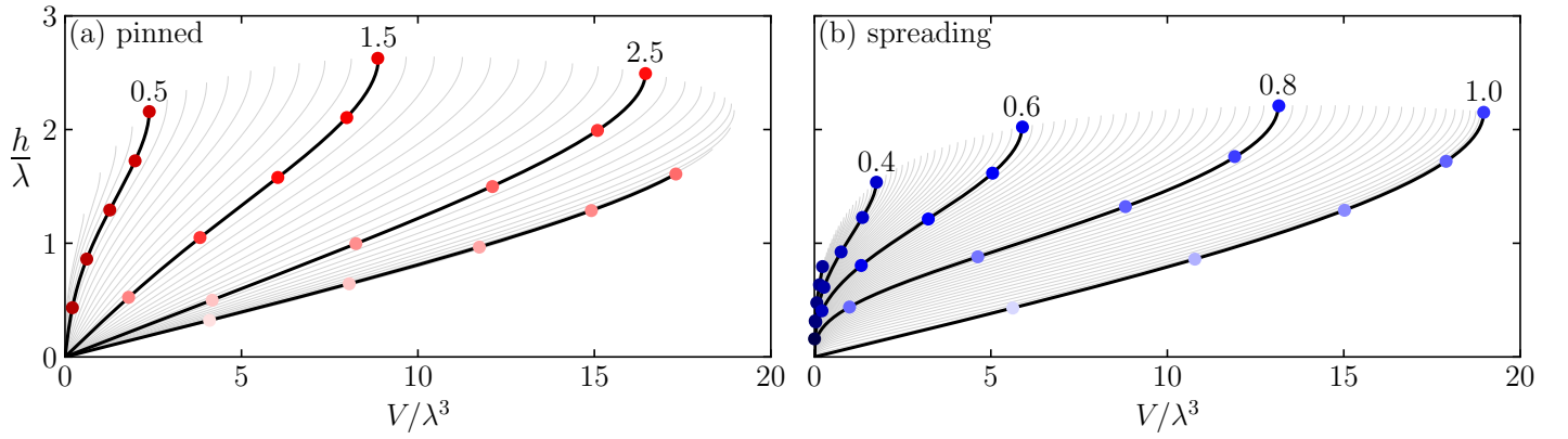
Figure 2 Bubble height h and volume V . (a) Pinned bubbles with constant contact radius r_0 ; black lines are labelled with the value of r_0/\lambda . (b) Spreading bubbles with constant contact angle \phi_0 ; black lines are labelled with the value of \phi_0/\pi . Circle markers show the heights and volumes of the bubbles in Figure 1 using the same colour scale for R_h .
