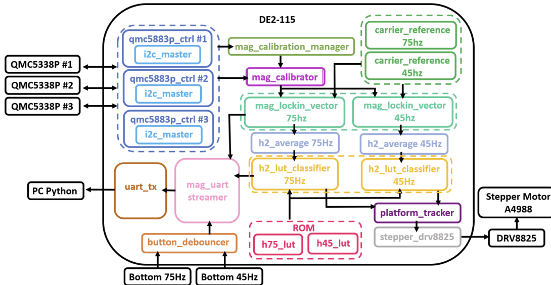
Figure 5: FPGA datapath architecture.
