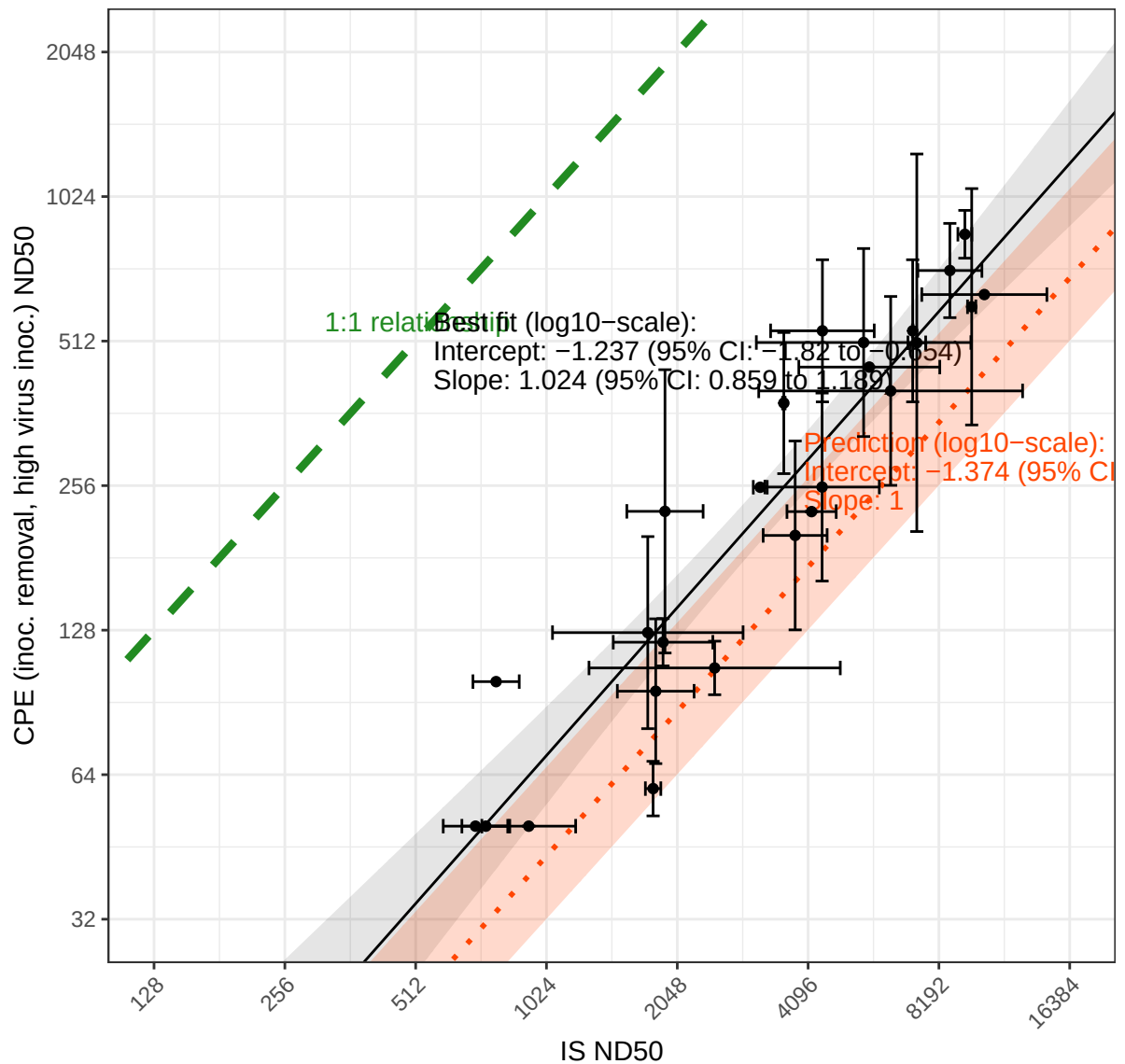
ND50 comparison: CPE (inoc. removal, high virus inoc.) vs IS
