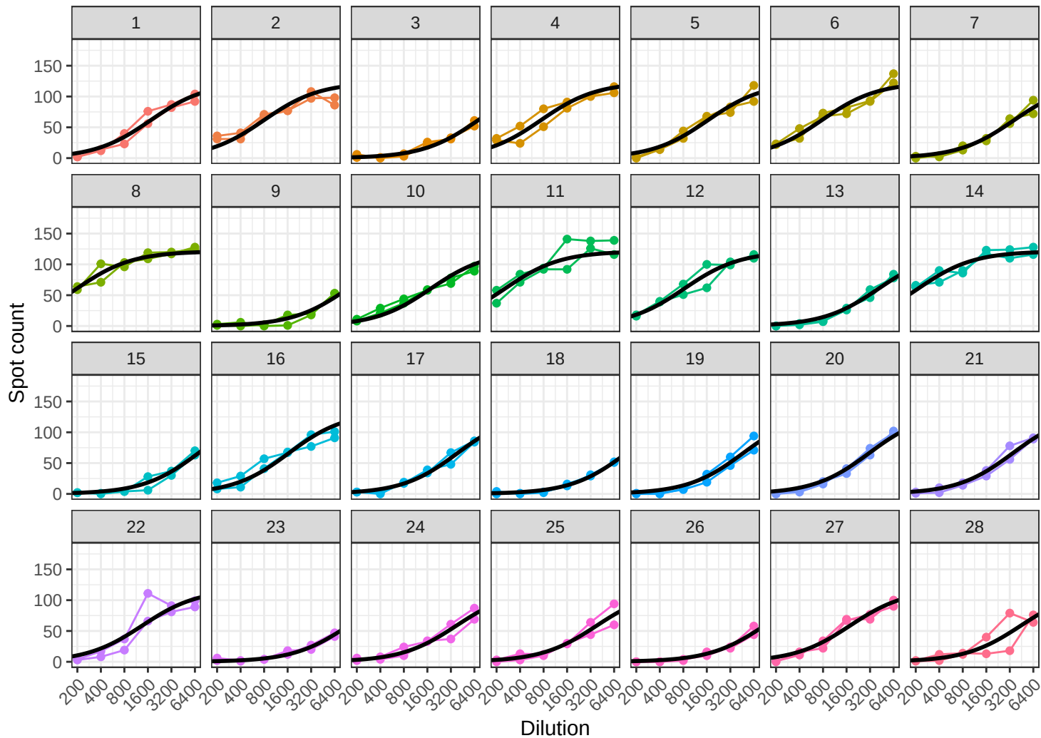
Fit to IS assay run 1
