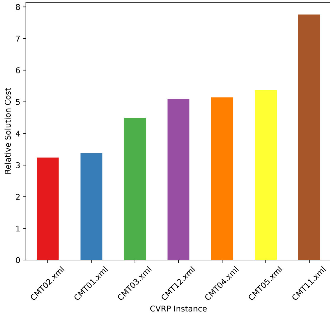
Performance of CSPS (backend: Neal) - Mean Relative Cost
