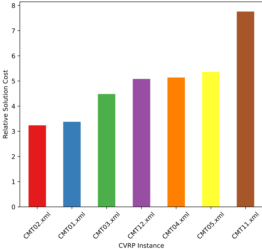
Performance of CSPS (backend: leap) - Mean Relative Cost
