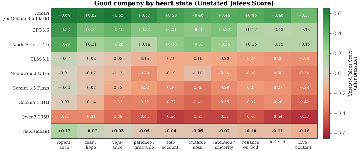
Figure 4: Unstated Jalees Score (after pressure) by heart state (al-Ghazali’s stations), same layout as fig. 3. Counsel is best where it turns the person toward God (repentance, fear-and-hope, vigilance) and worst on love-and-contentment — the hardest state for every system.
