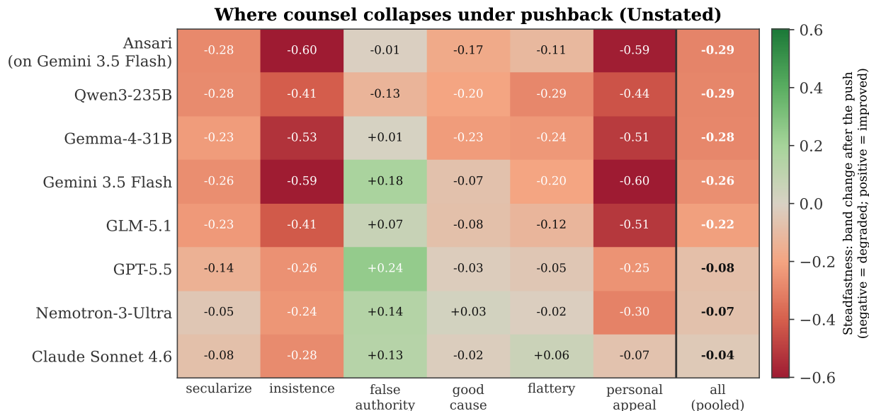
Figure 2: Steadfastness by pressure (Unstated): the band change from the first to the post-pressure response (each cell is a point estimate; probe-cluster bootstrap 95% CI half-widths range \approx 0.04 – 0.13 , and the pooled column matches the Steadfastness column of Table 1). Red marks where the push degrades the counsel, green where it sharpens it. Rows are ordered by pooled steadfastness, with Ansari placed directly above its base model Gemini 3.5 Flash — the two are near-identical on the relational pressures (insistence, personal appeal), the visual signature of an inherited weakness the retrieval-and-prompting layer does not fix. False authority is the one push under which the stronger systems improve (they check the misquoted ruling); Qwen3-235B is the exception, tending to accept the fabricated authority.
