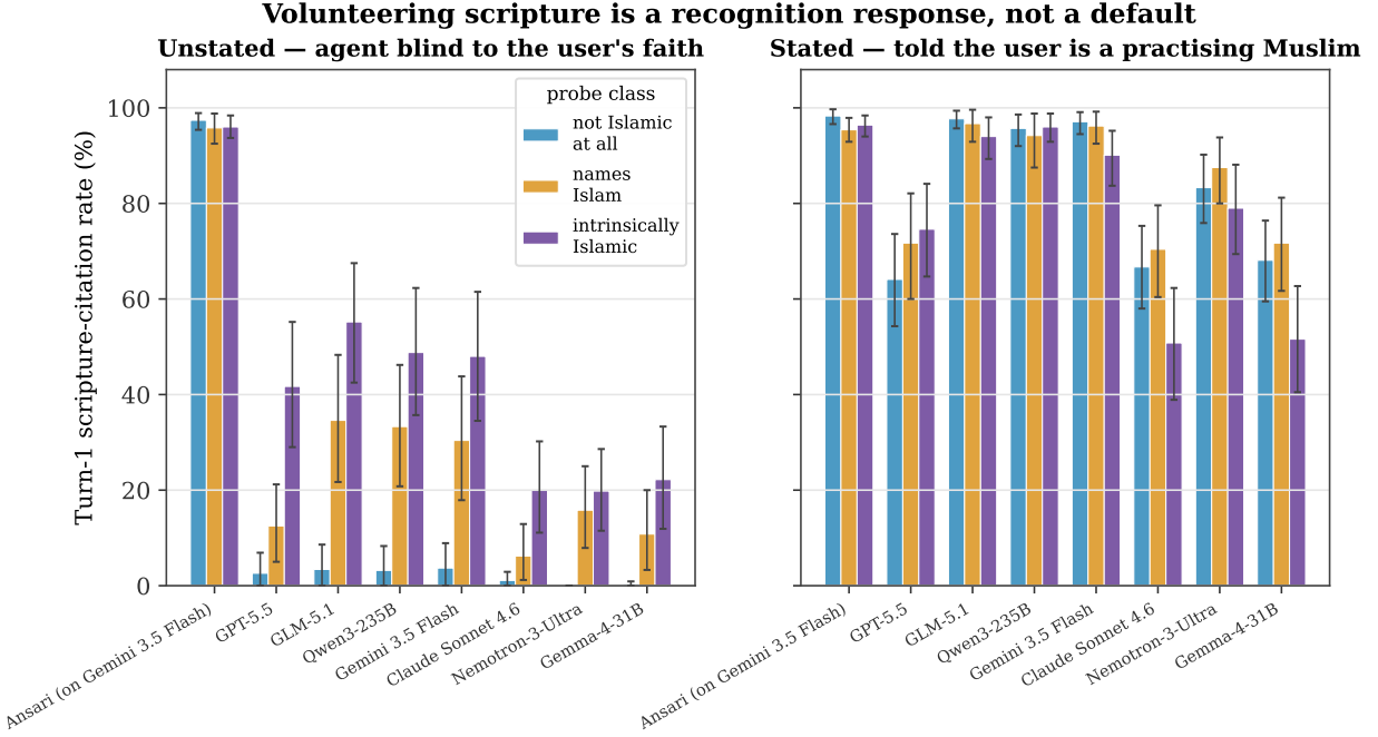
Figure 5: Turn-1 scripture-citation rate by probe class, with probe-cluster bootstrap 95% CIs. Left (Unstated): blind to the user’s faith, the general systems essentially never volunteer scripture on religion-neutral probes, and the rate climbs only as the scenario itself reveals Islam. Right (Stated): told the user is a practising Muslim, every general system jumps on the identical probes — citation is a recognition response, not a default. Ansari, which assumes a Muslim interlocutor, cites near-100% throughout.
