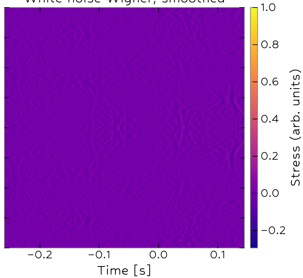
White noise Wigner, smoothed
