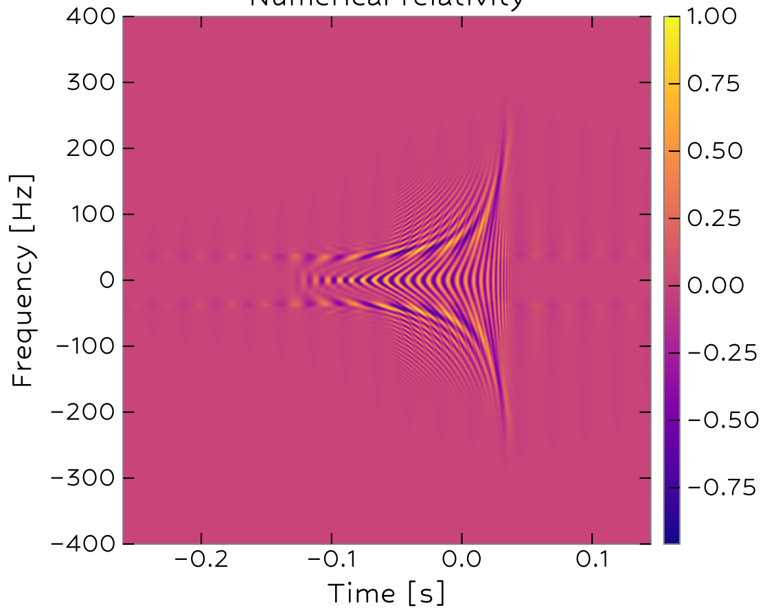
Numerical relativity
