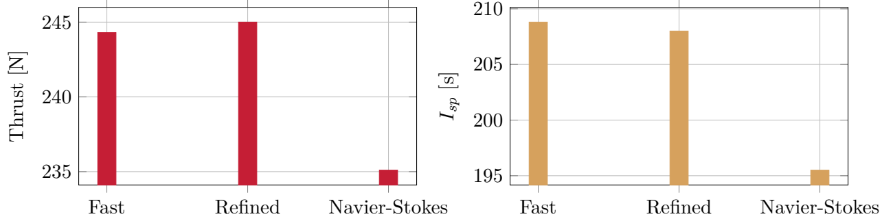
Figure 12: Flow-mode comparison for the packaged sample case. The final app solve uses the Navier-Stokes path.
