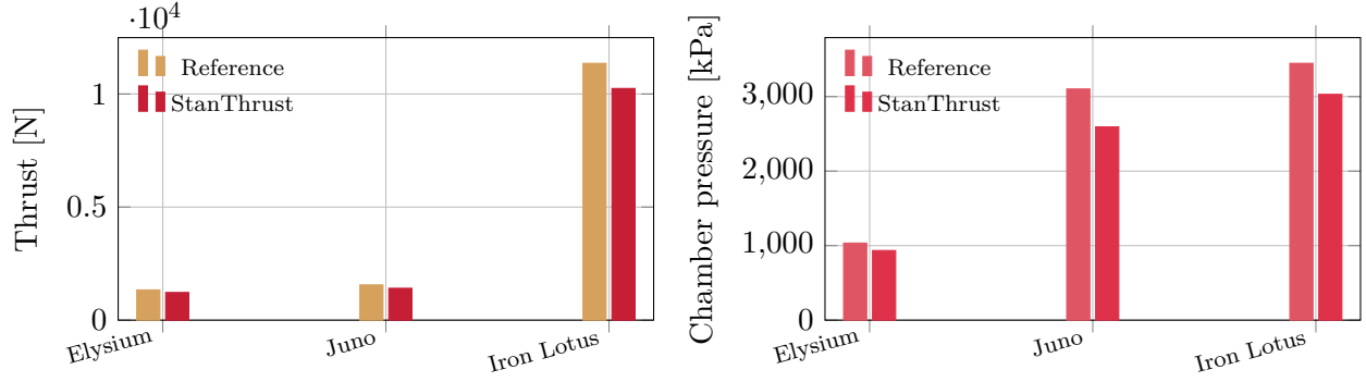
Figure 19: Published operating-point anchors versus StanThrust reconstructed operating points.
