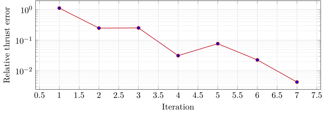
Figure 14: Default-case convergence trace of the chamber iteration. The current report case converged in 7 iterations.
