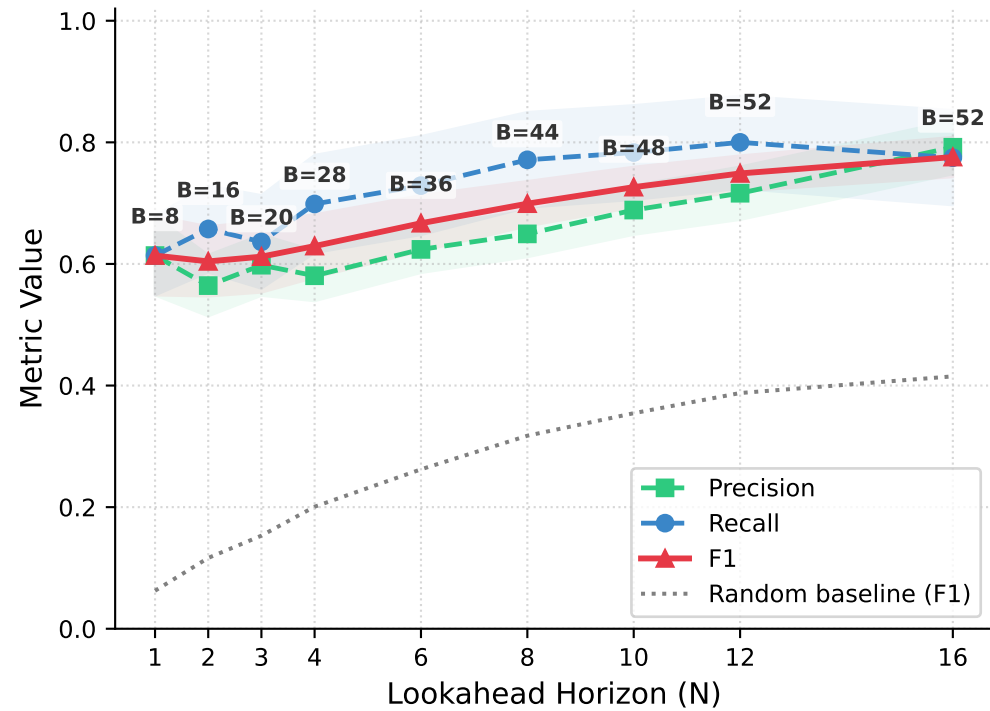
Embeddings only
