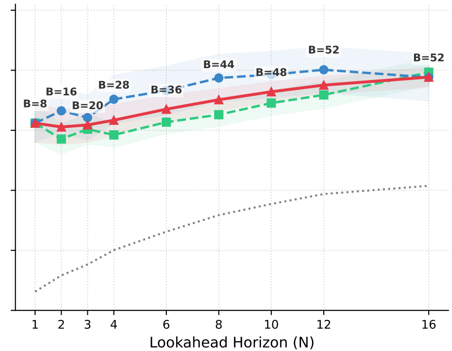
Embeddings + Markov
