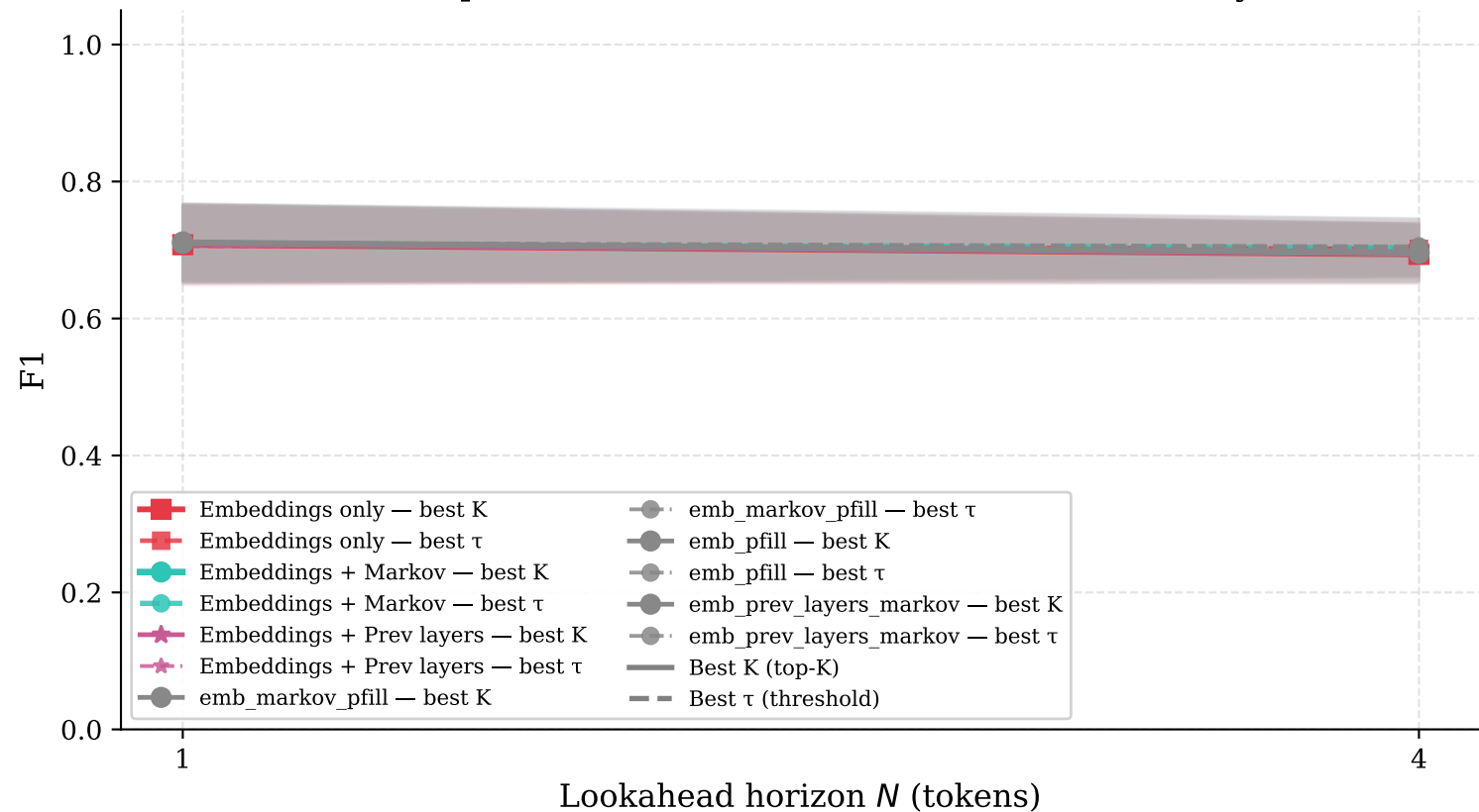
Oracle Best-K vs Best- \tau F1 per Horizon (solid = top-K, dashed = threshold; mean \pm std over layers)
