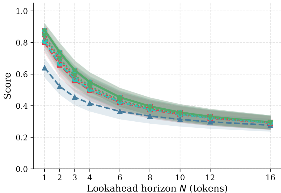
Recall@16
