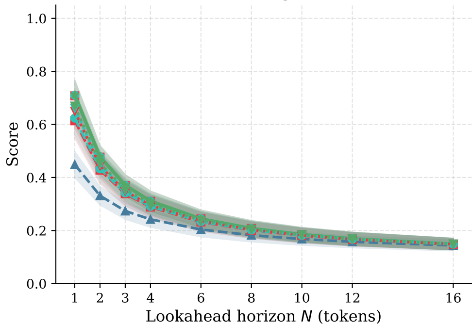
Recall@8
