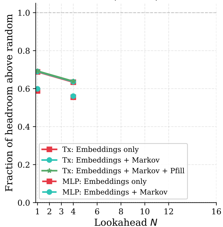
(c) Normalized Skill (F1 - \rho) / (1 - \rho)
