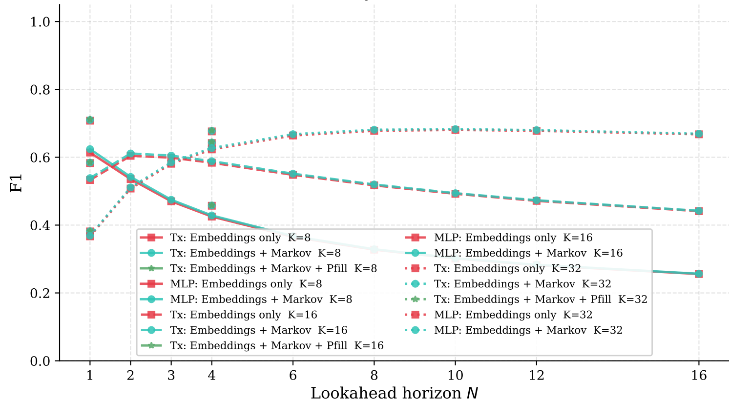
Fixed-K F1 vs Horizon — Ablation (mean over layers, K \in [8, 16, 32] )
