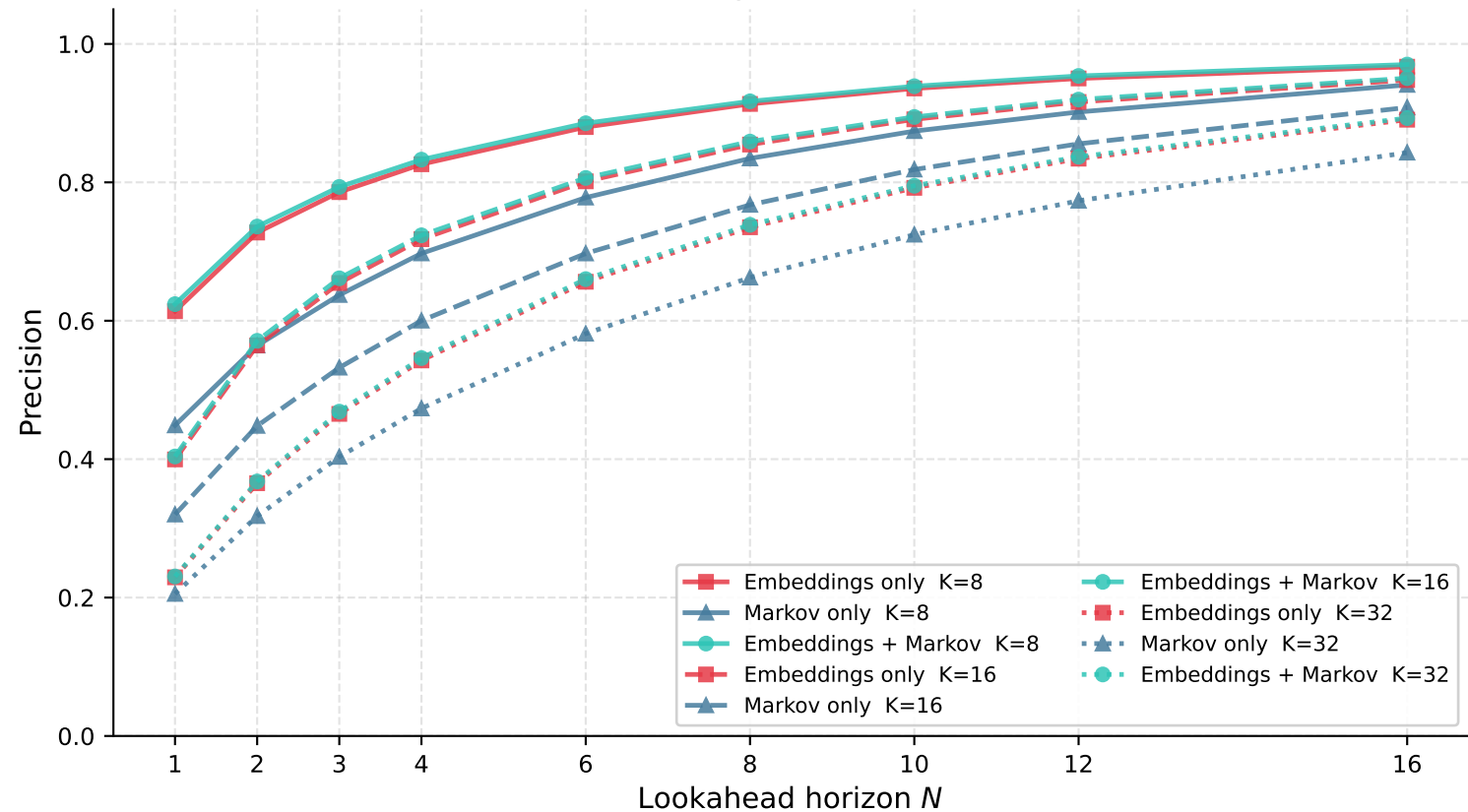
Fixed-K Precision vs Horizon — Ablation (mean over layers, K \in [8, 16, 32] )
