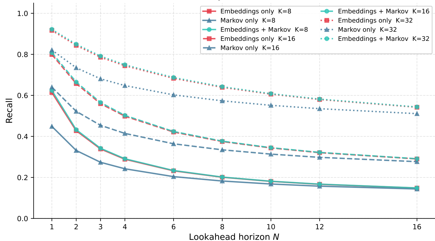
Fixed-K Recall vs Horizon — Ablation (mean over layers, K \in [8, 16, 32] )
