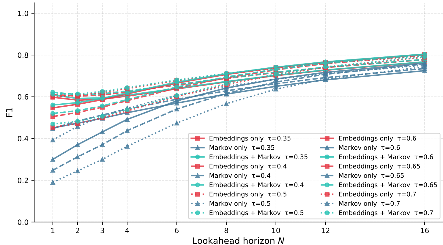
Threshold F1 vs Horizon — Ablation (sigmoid \geq \tau , mean over layers)
