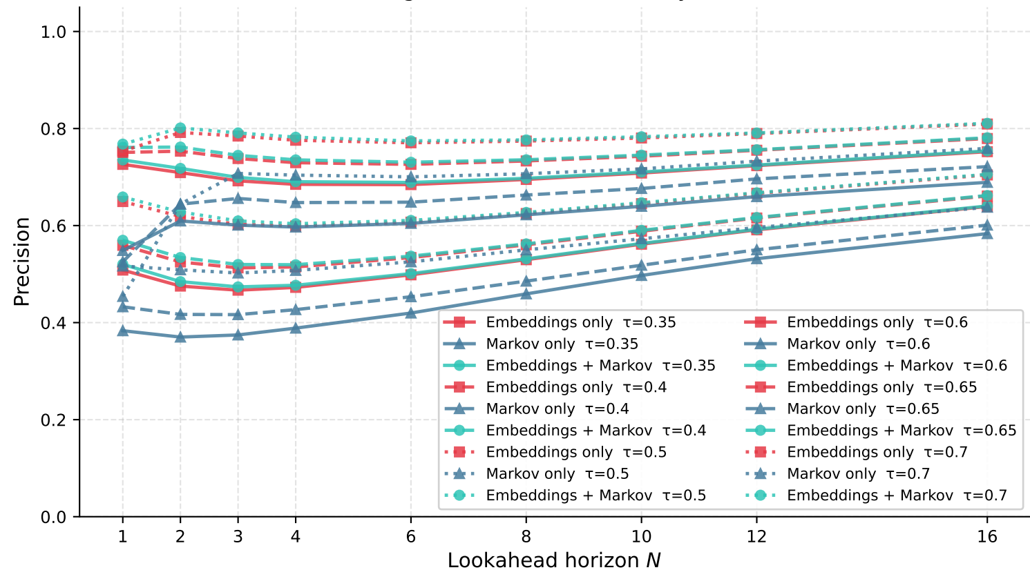
Threshold Precision vs Horizon — Ablation (sigmoid \geq \tau , mean over layers)
