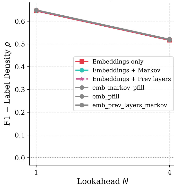
Disentangling predictor skill from label-density confound (mean over decoder layers) (b) Absolute Skill F1 - \rho
