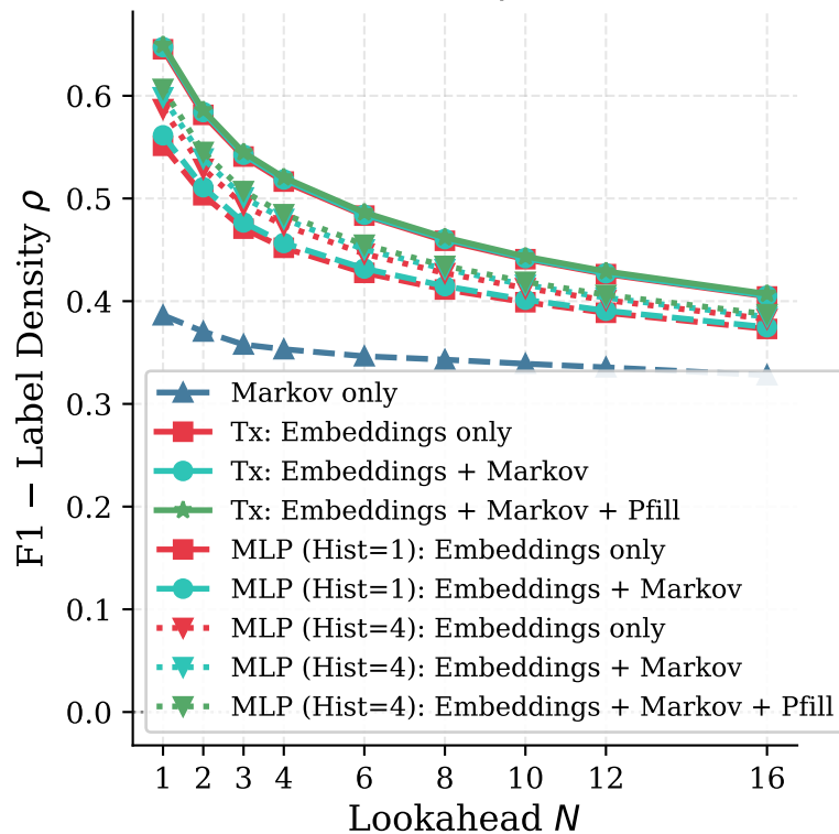
Disentangling predictor skill from label-density confound (mean over decoder layers) (b) Absolute Skill F1 - \rho
